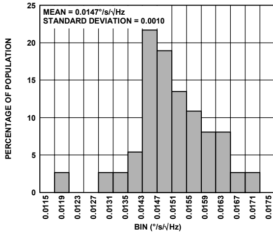
Figure 11. Noise Histogram
