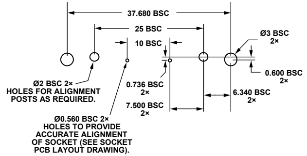
Figure 18. Interface Board Hole Locations for Bulkhead Mount
