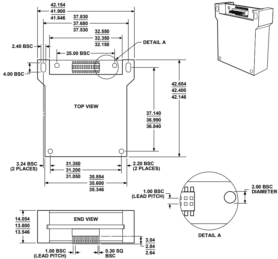
Figure 20. ADIS16120 PCB Module with Connector Interface (ML-24-1) Dimensions shown in millimeters
