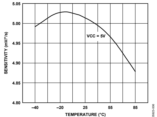
Figure 6. Gain Sensitivity vs. Temperature @ ±300°/sec
